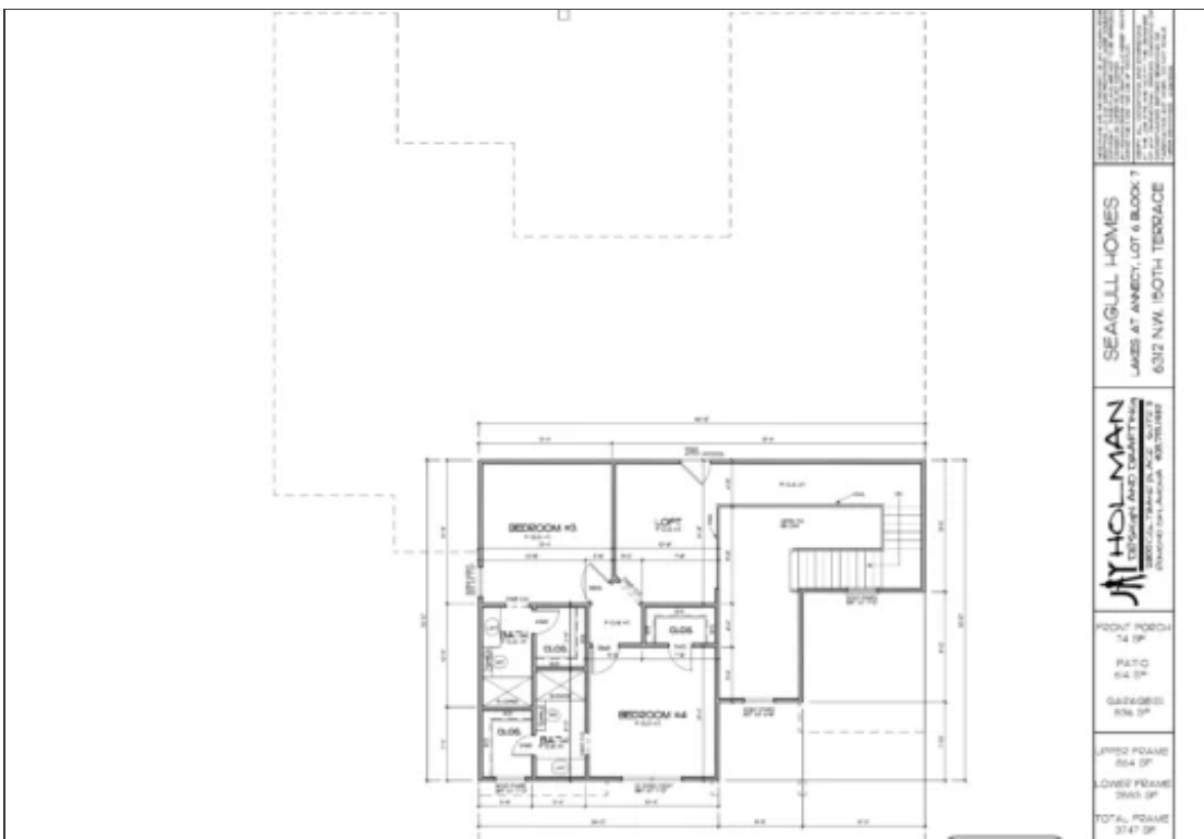
Floor Plan (2)
